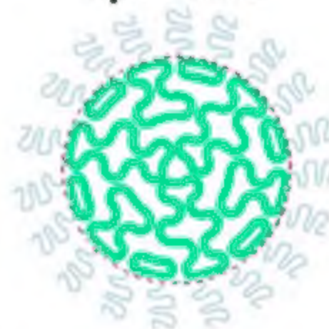
cubosome
